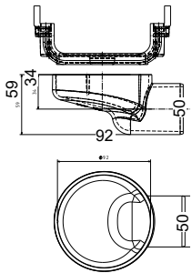
Drain connection ring NW 50 with lateral outlet
