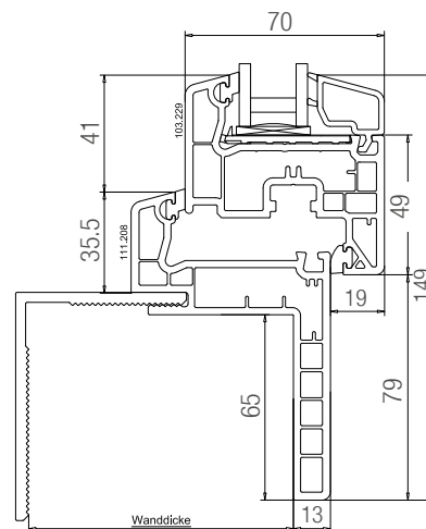
Drawing: Klickfix 70 - TOP and MDK
