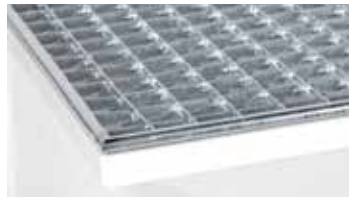
Pressure-locked edge protection grating Mesh width 30/30 for loads up to 6.2 kN
