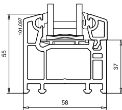
Profile cross-section FIB 58 58 mm installation depth
