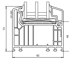
Profile cross-section FIB 82 82 mm installation depth
