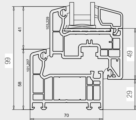
Profile cross section WOLFA MKD windows De Luxe 70 with an installation depth of 70 mm
