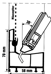
Profile cross-section Type PLUS
