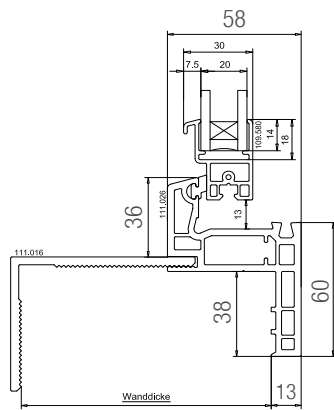
Drawing: Klickfix 58- PLUS
