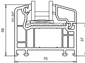
Profile cross-section FIB 70 70 mm installation depth
