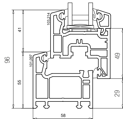
Profile cross section WOLFA MKD windows Klassik 58 with 58-mm installation depth
