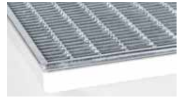
Pressure-locked edge protection grating Mesh width 30/10 for loads up to 7.2 kN (car-trafficable)
