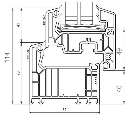
Profile cross section WOLFA MKD windows De Luxe 82 with an installation depth of 82 mm
