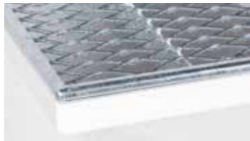
Expanded metal edge protection grating for loads up to 4.7 kN
